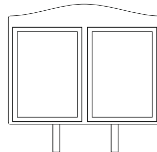
1630mm x 1210mm aluminium board - curved or flat top 2 x 9A4 poster cases 2 x 76mm diameter aluminium posts £1250.00 + vat
